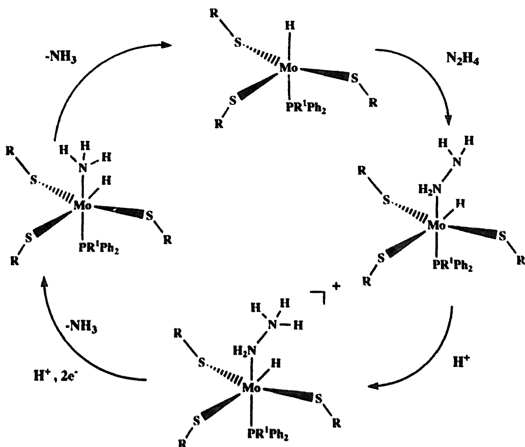
Fig. 10. Scheme of reduction of hydrazine by the complexes [\text{MoH}(\text{SR})_3(\text{PR}'\text{Ph}_2)] ( \text{R} = \text{C}_6\text{H}_2\text{Me}_3\text{-2,4,6} or \text{C}_6\text{H}_2\text{Pr}_3\text{-2,4,6} ; \text{R}' = \text{Me} or \text{Et} ).
