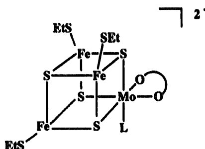
Fig. 8. Cluster anions which model the coordination environment of Mo in FeMoco ( \text{L} = \text{MeCN} , imidazole, etc.; \text{O}-\text{O} = \text{C}_6\text{Cl}_4\text{O}_2^{2-} )
