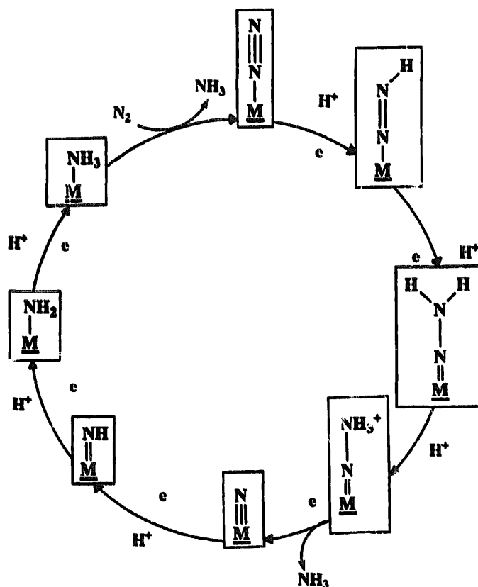
Fig. 3. Reduction of \text{N}_2 at tertiary phosphine sites. \underline{\text{M}} = \text{M}(\text{diphosphine})_2 , where \text{M} = \text{Mo, W, V or Fe} .
