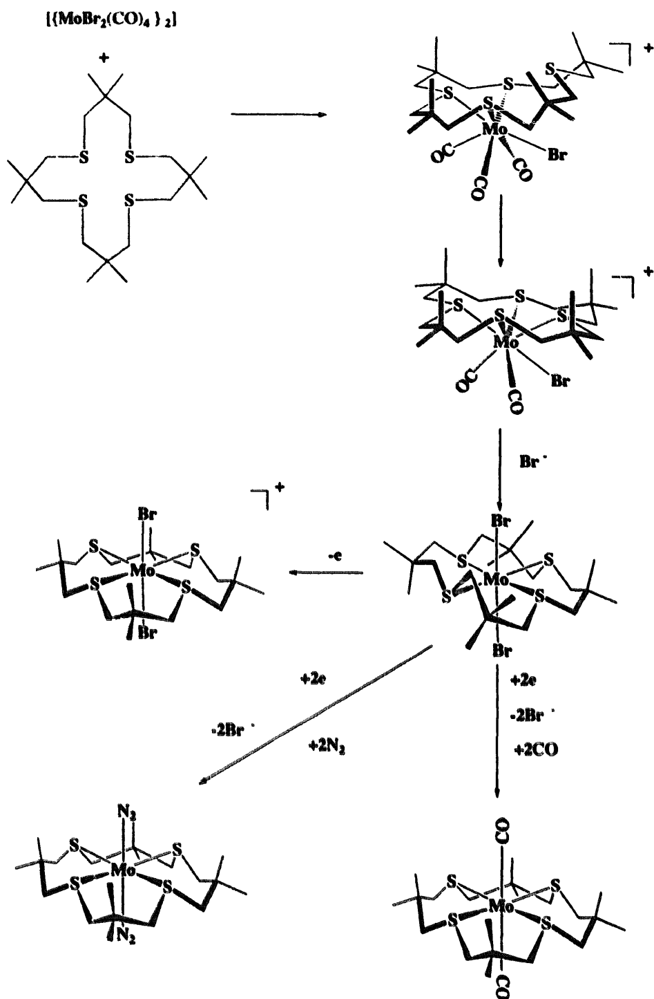
Fig. 6. General scheme of preparation of complexes of \text{Me}_8\text{16[ane]S}_4 . Parts of the macrocyclic ligand are omitted for clarity.
