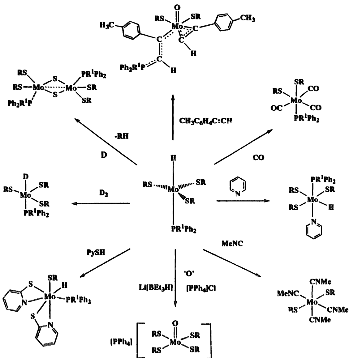
Fig. 9. General scheme of reactions of the complexes [\text{MoH}(\text{SR})_3(\text{PR}^1\text{Ph}_2)] ( \text{R} \rightleftharpoons \text{C}_6\text{H}_2\text{Me}_3\text{-2,4,6} or \text{C}_6\text{H}_2\text{Pr}^i\text{-2,4,6} ; \text{R}^1 \rightleftharpoons \text{Me} or \text{Et} ).
